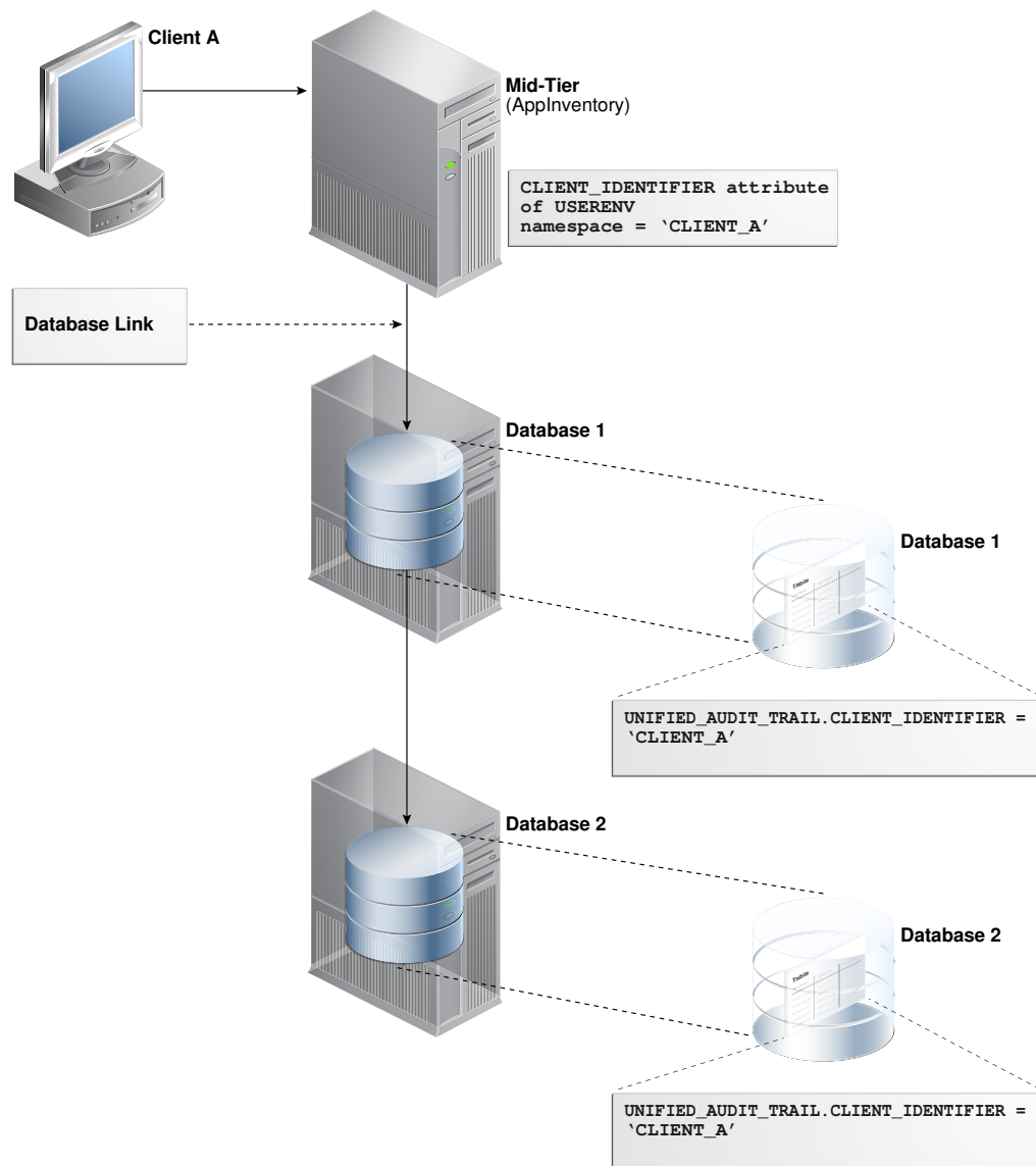
Figure 25-2 Auditing Client Identifier Information Across Sessions
