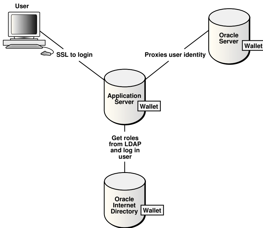
Figure 3-2 Multitier Authentication
