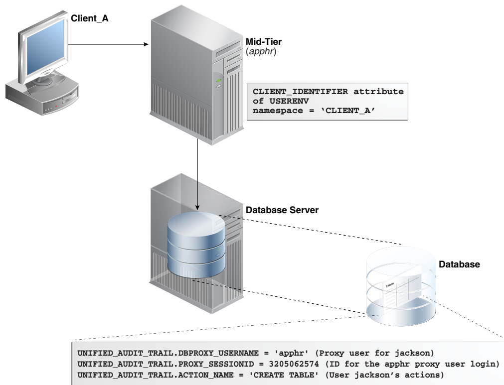
Figure 25-1 Auditing Proxy Users
